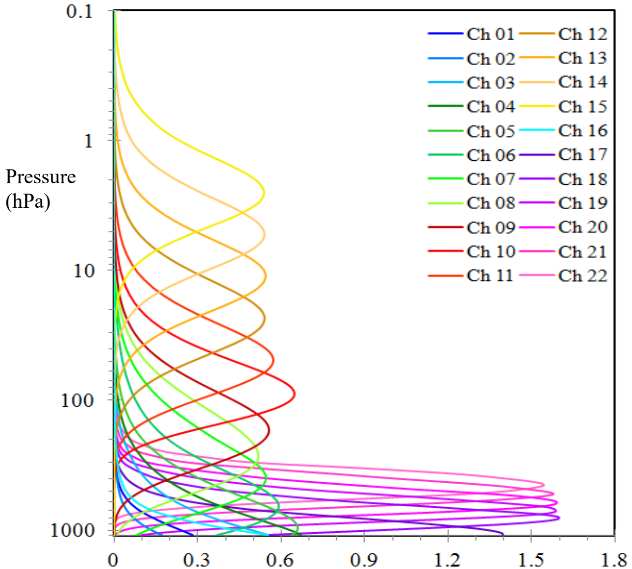
Figure 1: ATMS Weighting Functions
