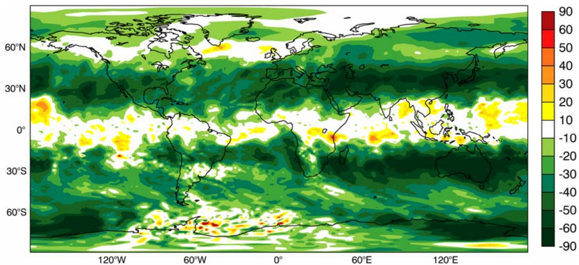
Figure 7: Differences in the root mean square (RMS) of the humidity increments at model level 21 (approx. 44 hPa) between the experiment RAD-2d and the RAD experiment, relative to the RMS of the increments in RAD [%]. Green areas indicate a reduction of increments from using the 2d-operator.
