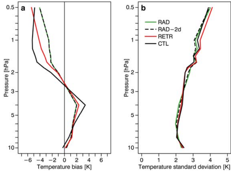
Figure 2: Comparison between HALOE temperature retrievals over the tropical region (0-20S) against analyses from the CTL (solid black), RAD (solid green), RAD-2d (dashed black), and RETR (solid red) experiment. The data covers the period 1-29 September 2003 (70 profiles), and the two panels show the bias (a) and the standard deviation (b) of the retrieval minus analyses differences.
