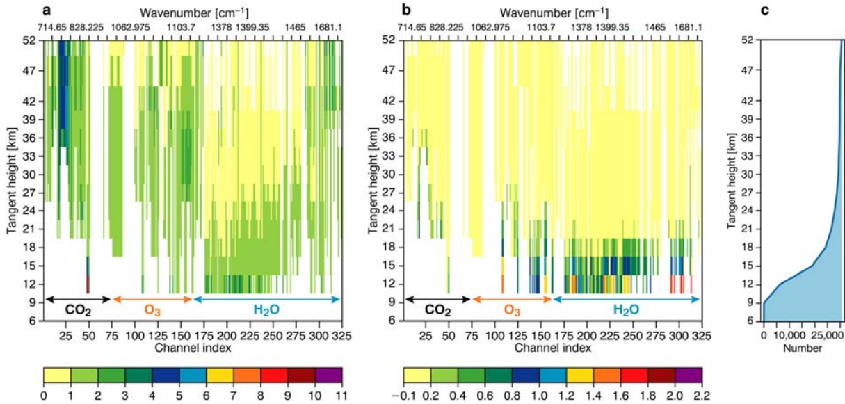
Figure 6: a) Standard deviation of observation minus First Guess departures for used MIPAS radiances from the experiment RAD-2d as a function of channel index and nominal tangent altitude. The values have been normalised by the instrument noise in each channel. Wavenumbers of selected channels are provided in the top axis for orientation. Correction of MIPAS radiance biases has been applied. b) Difference between the standard deviation of FG departures for the experiment RAD and the experiment RAD-2d as a function of channel index and nominal tangent altitude. The values have again been normalised by the instrument noise in each channel. c) Number of clear sweeps per tangent altitude.
