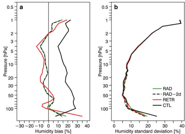
Figure 3: As Fig. 2, but for 195 SAGE II humidity retrievals over the North Polar region (60-74N), with values normalised by the mean retrieval value.
