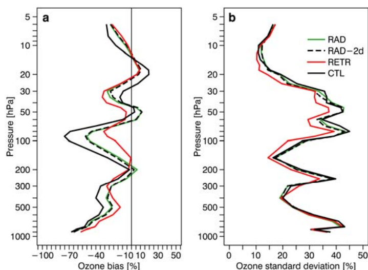
Figure 5: As Fig. 2, but for 49 ozone sondes over the South Polar region (60-90S), with values normalised by the mean retrieval value.
