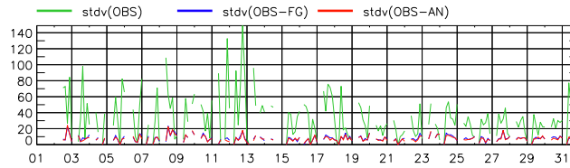
Figure 6: The time series of the standard deviation of the observations in the north polar region suggests that the enlarged variation seems to be generated mainly in the first half of the experimental period.
