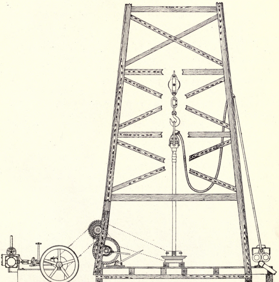
Rotary drilling rig. Engine to left of derrick and mud pump to right. Drill pipe passes through rotary table in center of derrick.
