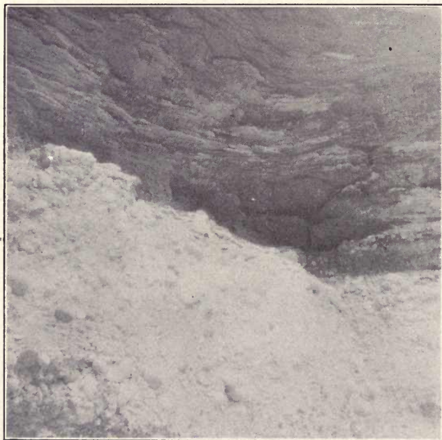
Seepages from top of Dakota and bottom of Benton formations, Alberta, Canada. These seepages have been exposed for thousands of years, hence the oil is inspissated and only the residue remains.
