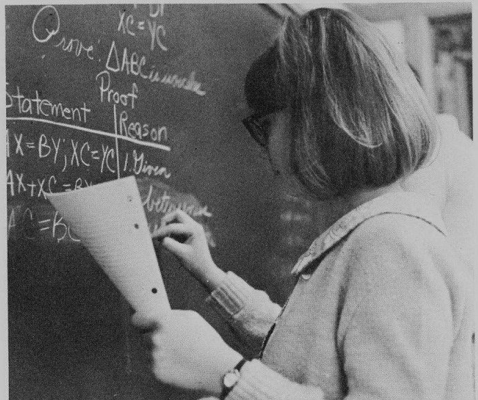
Pat Lange proves if AX = BY , then triangle ABC is isosceles.
