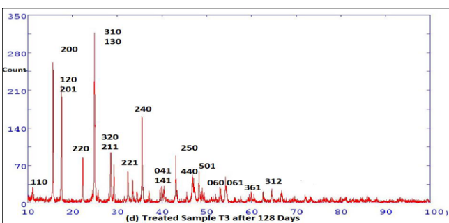
Figure 2d: XRD pattern of treated Sb_2S_3 sample T3 (128 days after biofield treatment).
