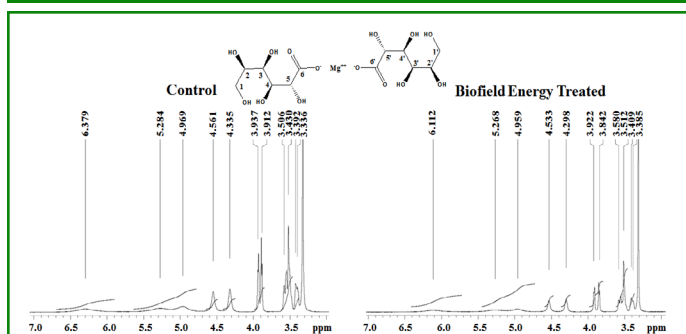
Figure 4: The ^1\text{H} NMR spectra of the control and Biofield Energy Treated magnesium gluconate.
