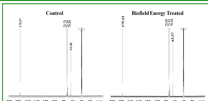
Figure 5: The ^{13}\text{C} NMR spectra of the control and Biofield Energy Treated magnesium gluconate.
