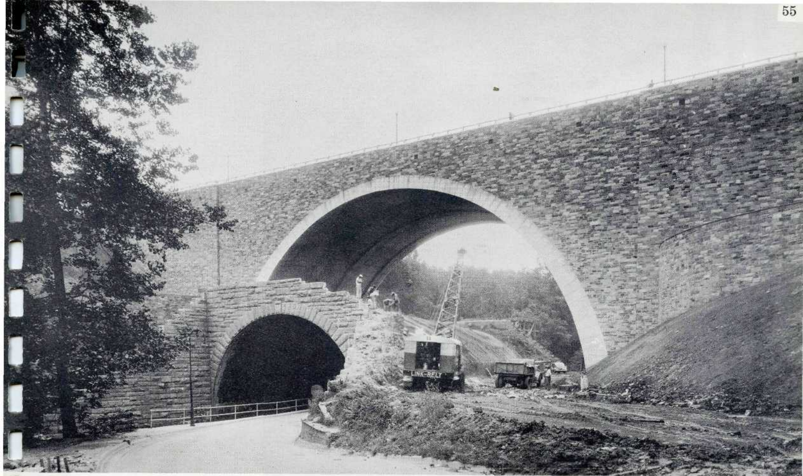
MASSACHUSETTS AVENUE BRIDGES—THE OLD AND THE NEW—1941 The obsolete, low-level culvert with its dangerous blind curve in the immediate approach to the tunnel being removed in the shadow of the new bridge.
